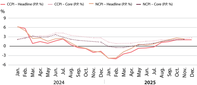
Inflation – CCPI & NCPI Graph – 02
